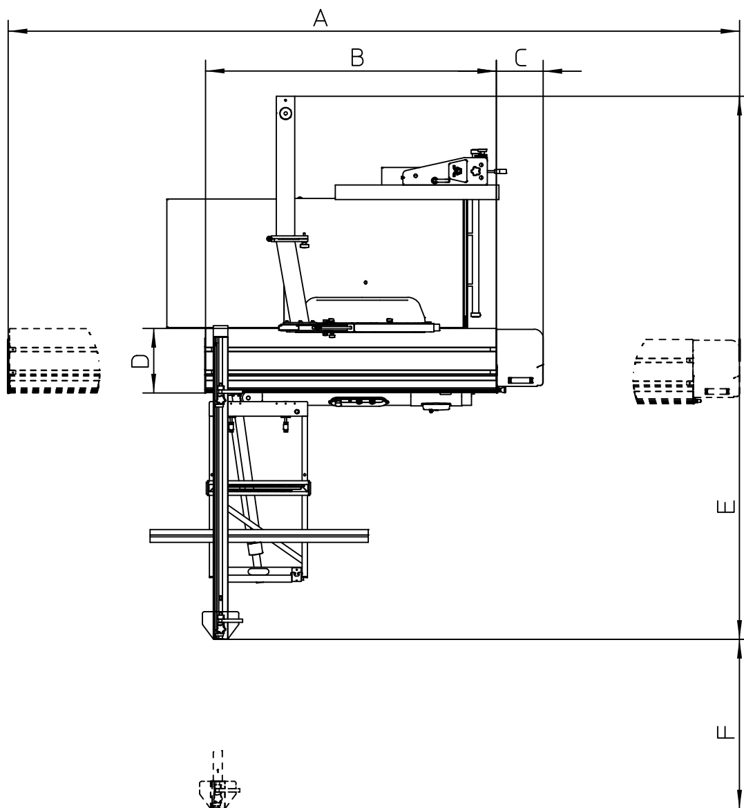
Footprint CZ300M II/ CZ300EL II
